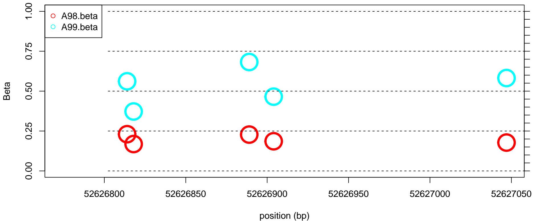
RegionID: 9625, chr12:52626814-52627047-Beta_values
