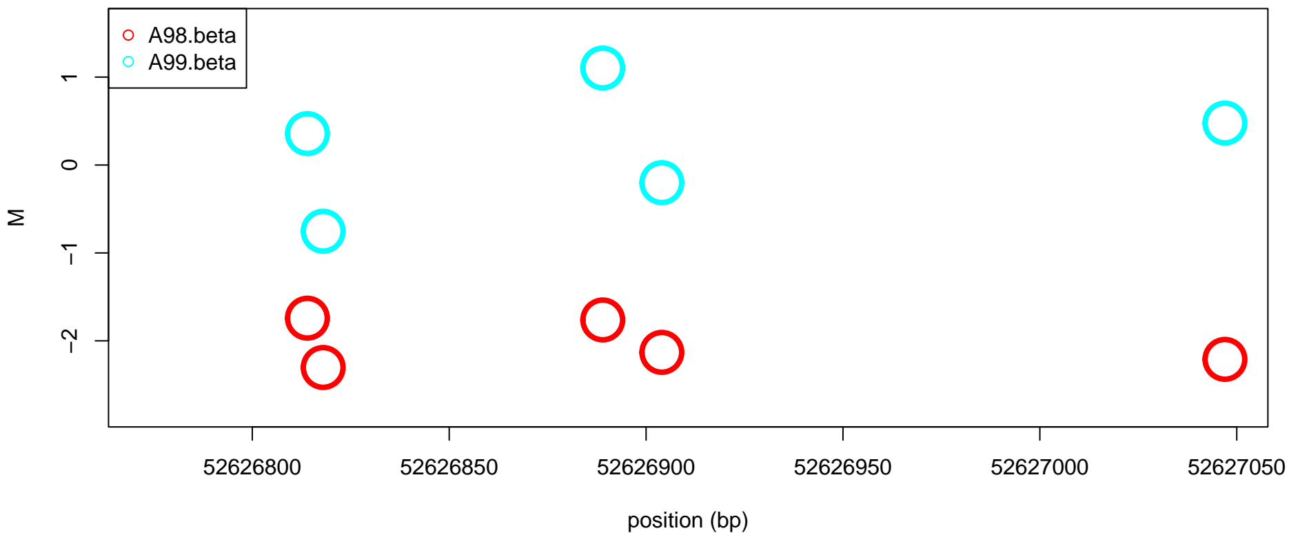
RegionID: 9625, chr12:52626814-52627047-M_values
